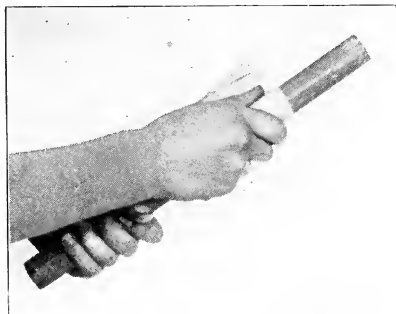
Fig. 129—Sandpapering Cylinder
